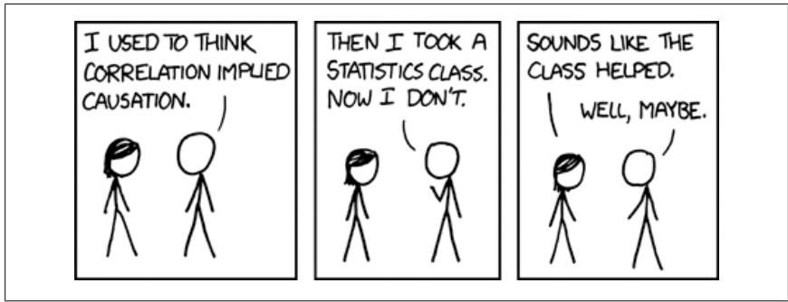
Figure 16-1. Correlation
