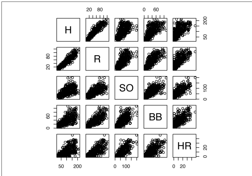
Figure 14-4. Pairs example
