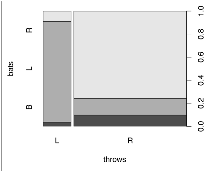
Figure 14-13. Spine plot
